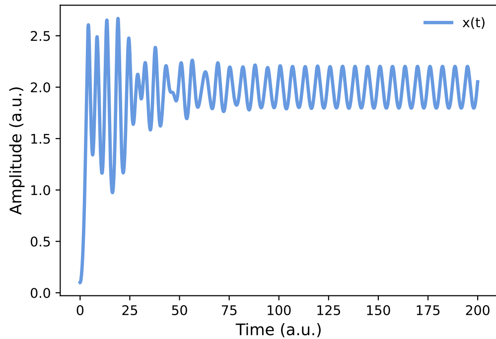
F_{ac}=0.5, F_{dc}=0.1, \omega=2
