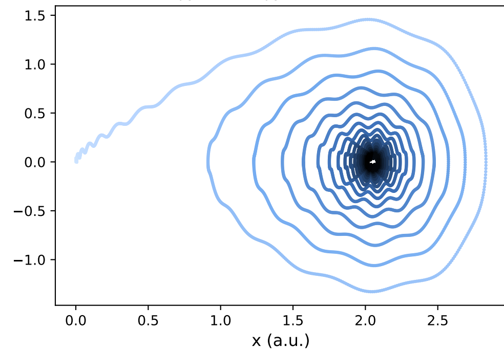
F_{ac}=0.5, F_{dc}=0.1, \omega=16
